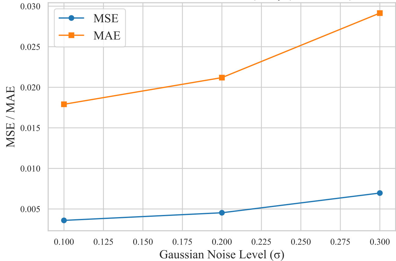
Noise Level vs. Reconstruction Quality (MSE, MAE)
